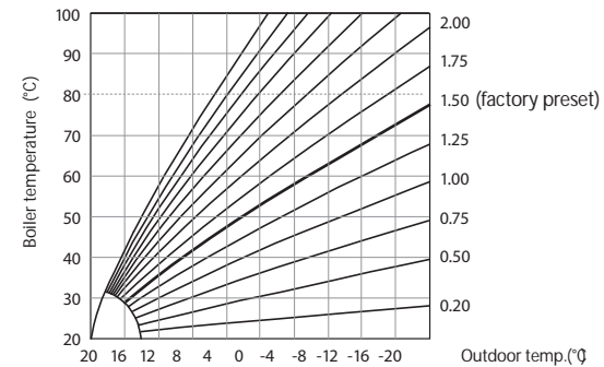
Diagram of heating curves
